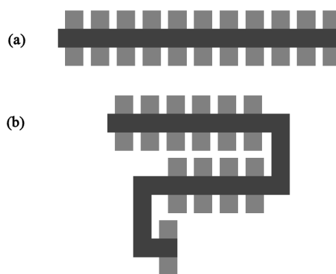
Figure 5. A page with 22 children drawn: (a) In the default shape, and (b) With the parent constraint. Although the bounding area of (b) is double that of (a), the aspect ratio is much smaller (1.0 vs. 5.1).
