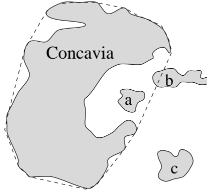
Figure 9. The convex hull of an island
