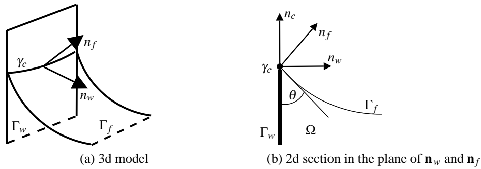
Figure 1. Geometrical description of the contact line
