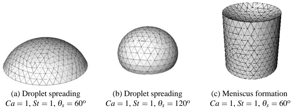
Figure 2. Computation to steady state with a specified static contact angle
