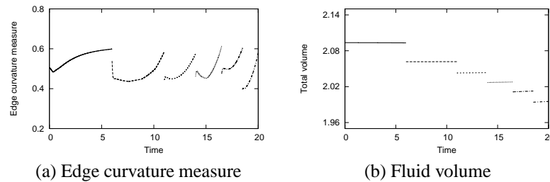
Figure 4. Statistics of the adaptive mesh procedure
