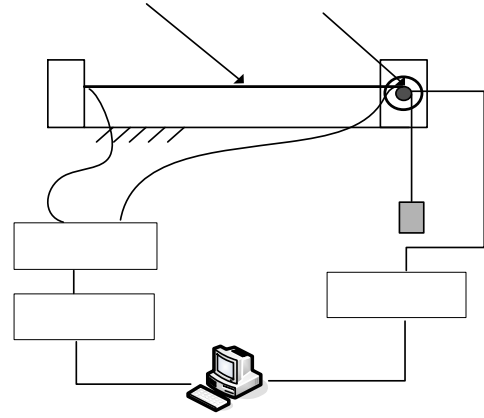
Fig. 10. Experimental apparatus.
