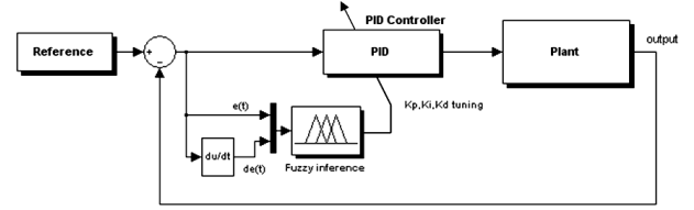
Fig. 1. Structure of self tuning PID controller.
