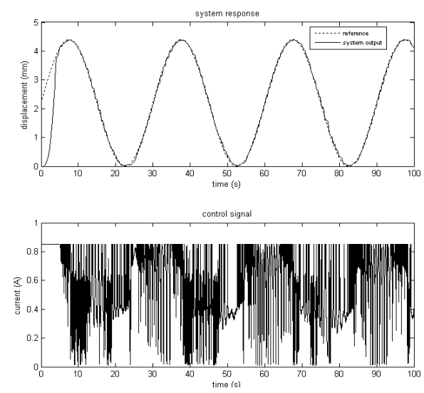
Fig. 16. System response with respect to sine reference input ( f = 0.033\text{Hz} ).
