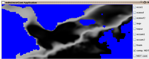
Figure 3: A fuzzy zero contour for the composite MDT dataset.
