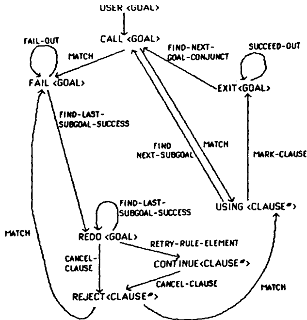
Figure 2. The correct interpreter.
