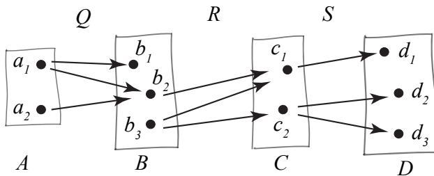
Fig. 1. Three relations between four times
