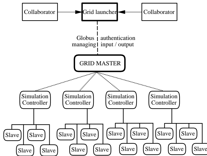
Fig. 5. Schematic of the Grid-enabled Optimisation PSE
